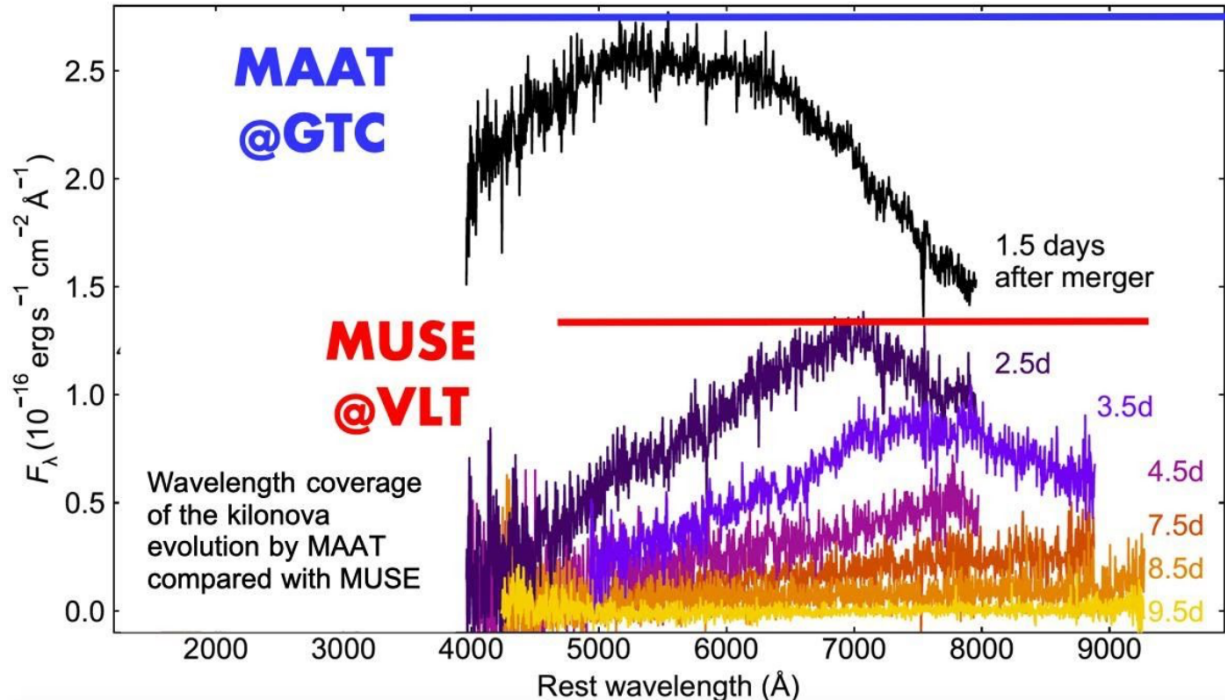
Figure 8. The spectral time series of kilonova AT2017gfo during the first 10 days of its emission (Pian et al. 2017). We highlight the broader wavelength coverage that can be observed with OSIRIS+MAAT (blue line), using a combination of the R1000B and R1000R grisms, as compared to MUSE (red line).
