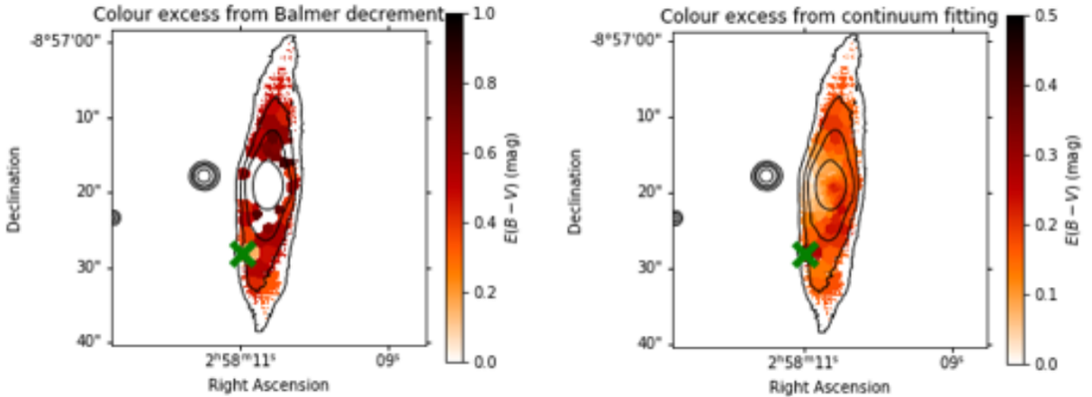
Figure 10. The distribution of the color excess E(B-V) obtained from the Balmer decrement ratio (left panel) and the fit of the stellar continuum (right panel) for the case of the host galaxy of GRB 100316D. The green cross corresponds to the location of the GRB.
