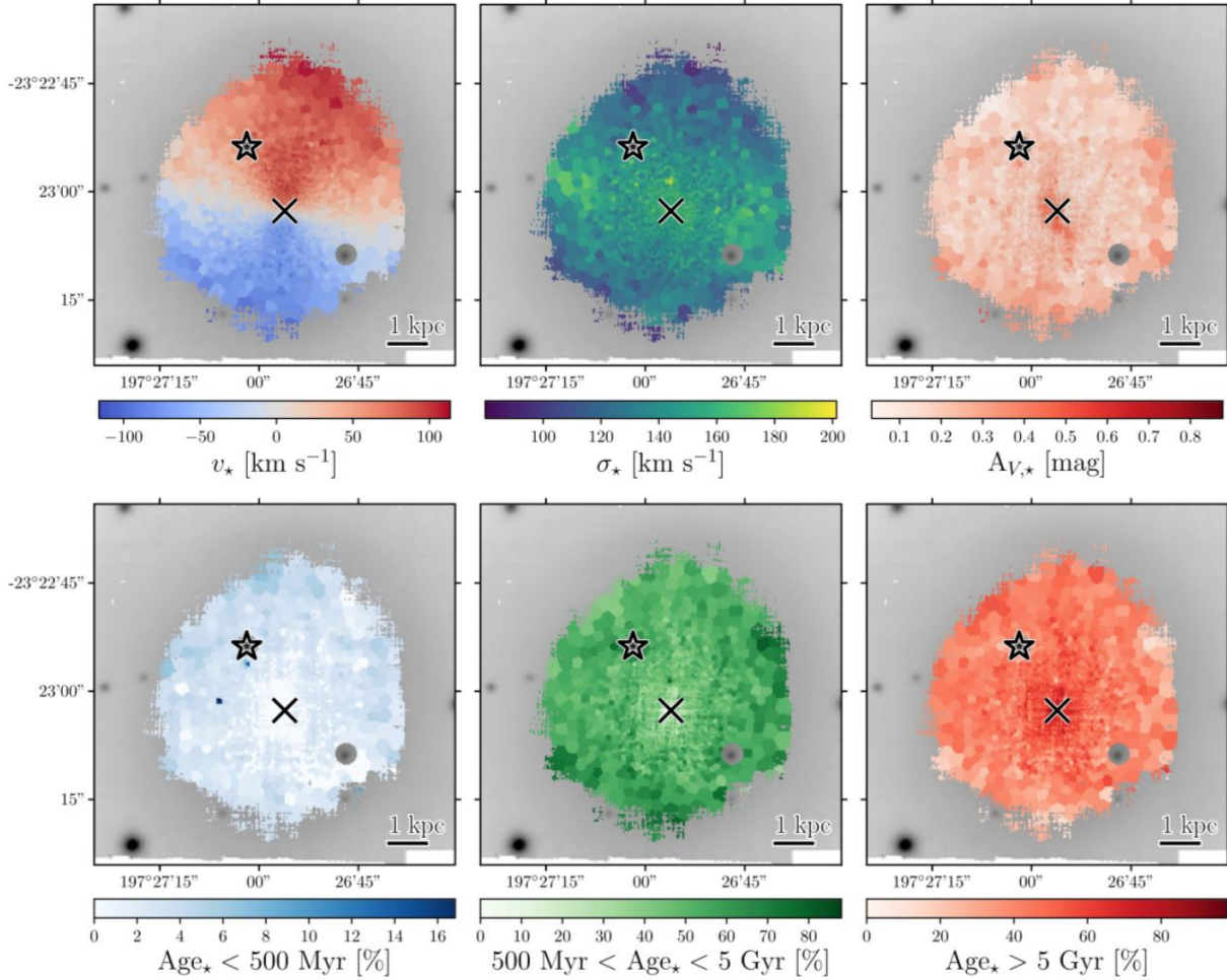
Figure 7. Stellar population map for NGC 4993 obtained with MUSE (Levan et al. 2017). The upper panels show the distribution of the radial velocities (left) as estimated from the stellar components for each single spectral bin, as well as its dispersion in terms of \sigma (middle) and the extinction as inferred from the fit continuum (right). Lower panels show the distribution of stellar ages for different age intervals: less than 500 Myr (left), between 500 Myr and 5 Gyr (middle) and larger than 5 Gyr (right). The black star corresponds to the location of the kilonova AT2017gfo.
