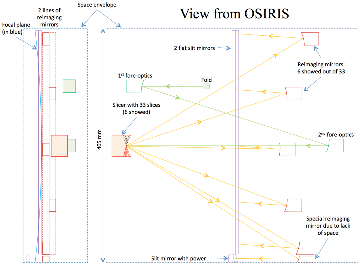
Figure 22. Optics lay-out of the proposed IFU concept.
