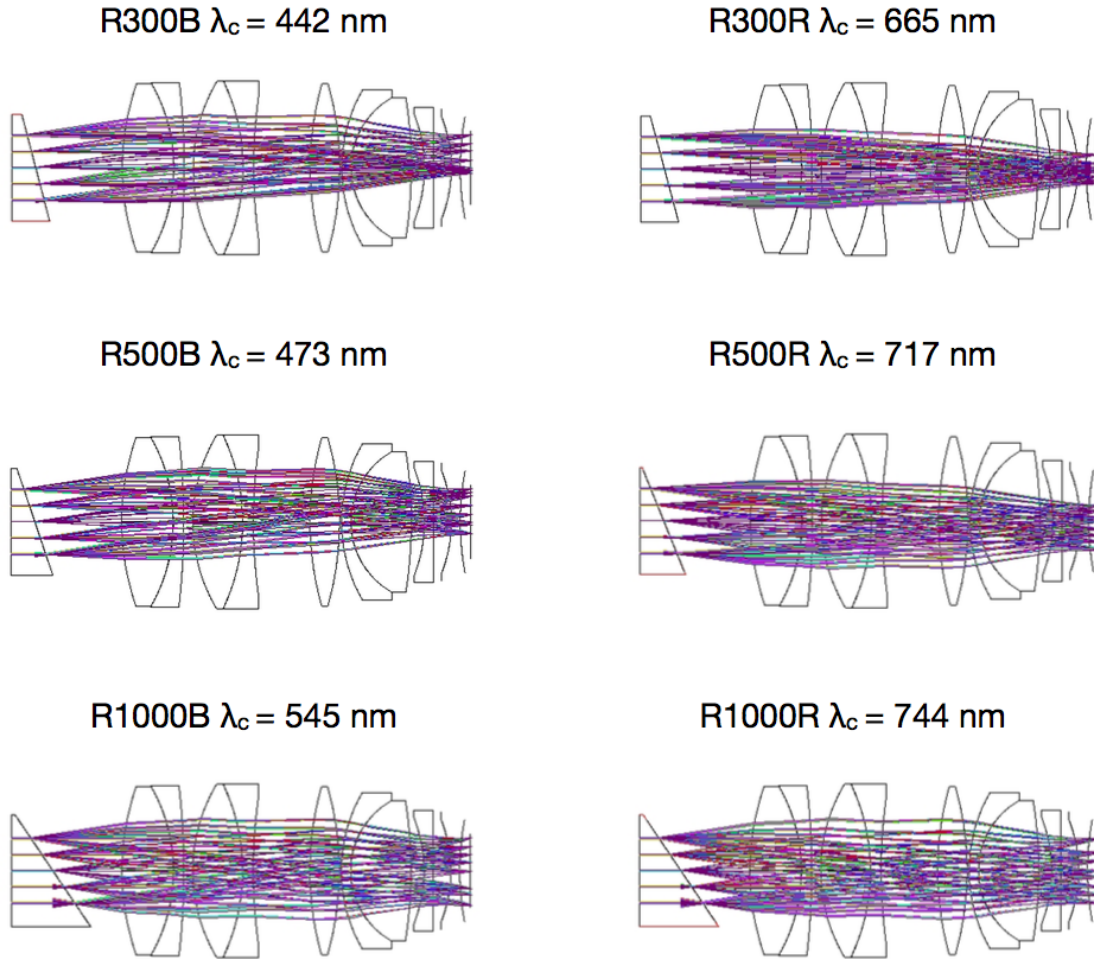
Figure 15. Zemax ray-tracing models of the OSIRIS suite of Grisms.
