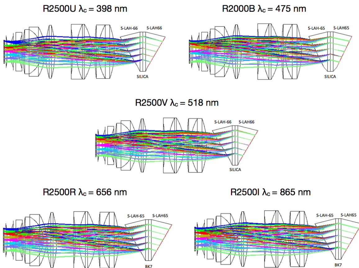
Figure 16. Zemax ray-tracing models of the OSIRIS suite of VPHs.
