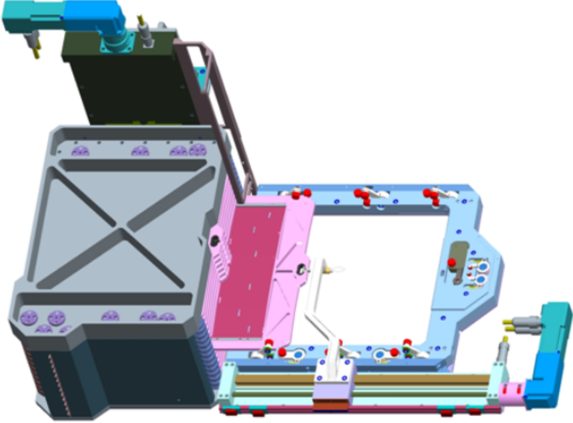
Figure 18. General view of the OSIRIS Slit Subsystem without baffle, consisting of a Jukebox (on the left in gray), with a capacity of 13 masks and a Charger, on the right in blue, which inserts the mask (in pink) selected by the control on the plane focal length of the telescope (Credit: GTC). The MAAT box will be inserted in the Jukebox and occupies the equivalent to 6 masks (see text). To all effects, the MAAT box will be inserted in the focal plane of OSIRIS when required as if it were another long-slit mask.
