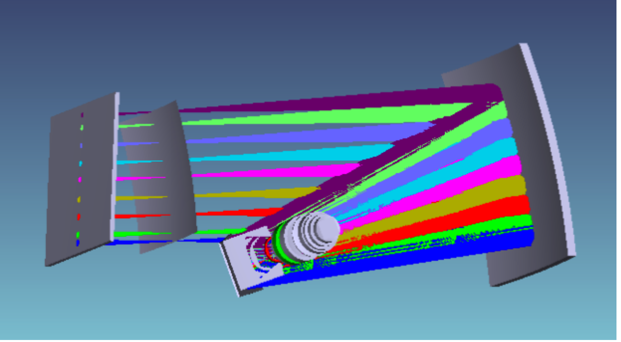
Figure 14. OSIRIS optical layout in spectroscopy mode.
