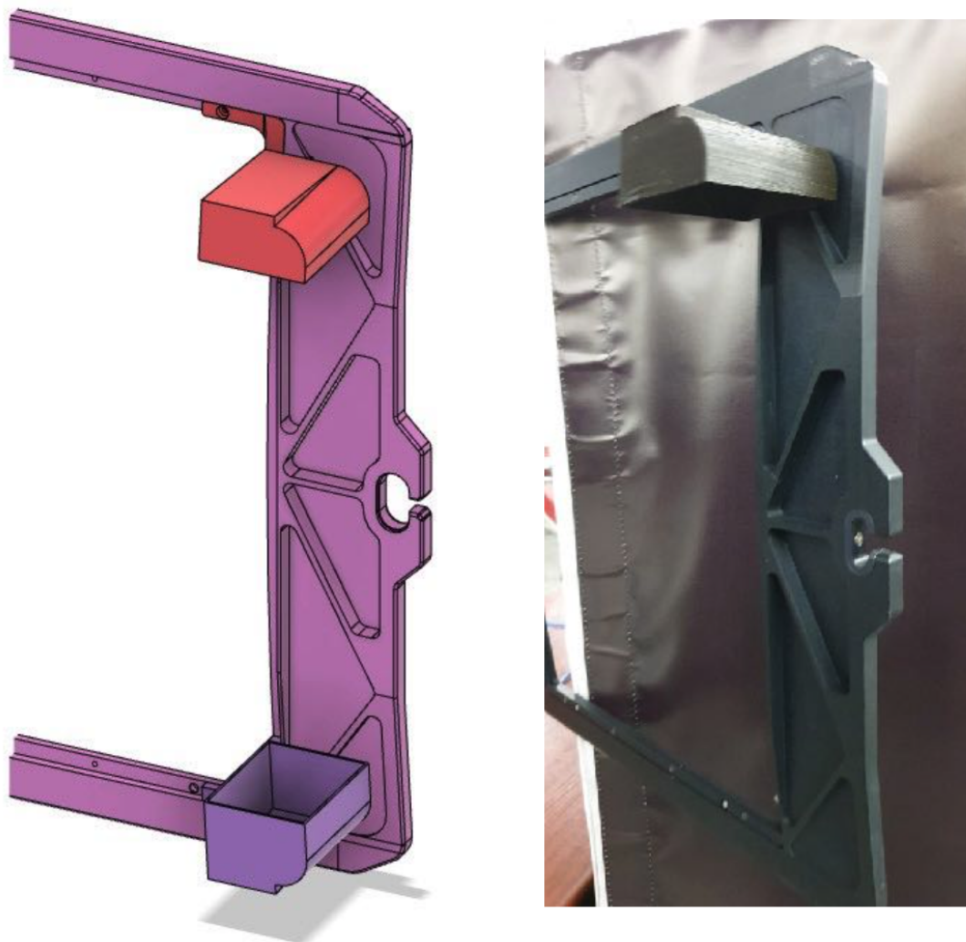
Figure 20. 3D printed dummies built for the in situ testing of the MAAT envelope on OSIRIS (Credit: GTC).
