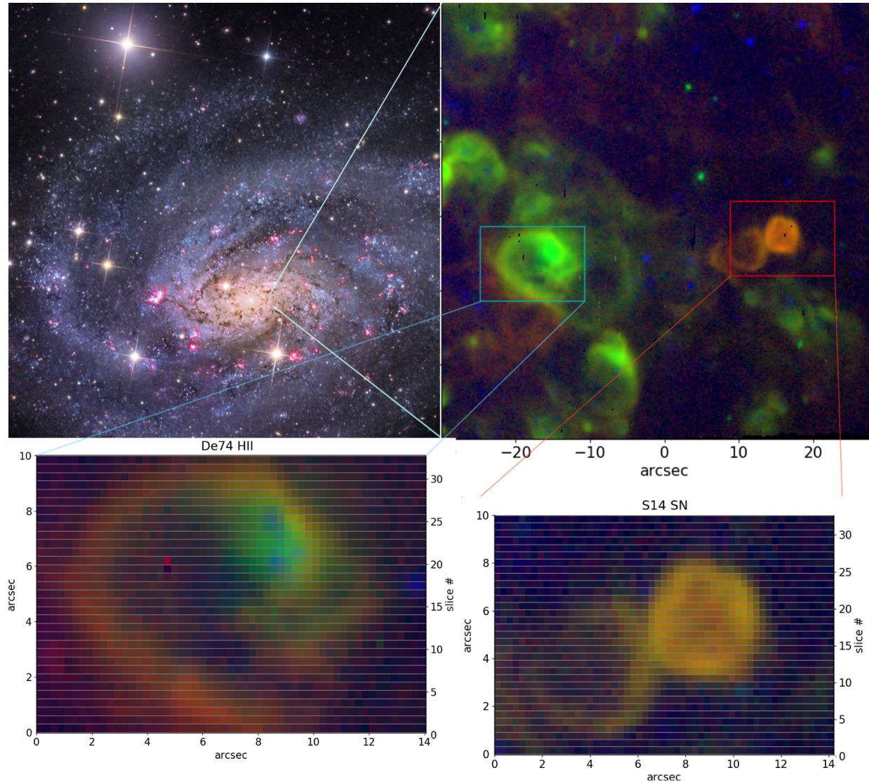
Figure 4. MAAT simulation of two nebular objects in the spiral galaxy NGC300. The HII region De74 (left) and the SN remnant S14 (right). The two bottom images show how the slicer sees each of the objects that are then dispersed onto the CCD to obtain the frames as in Figures 5 and 6.
