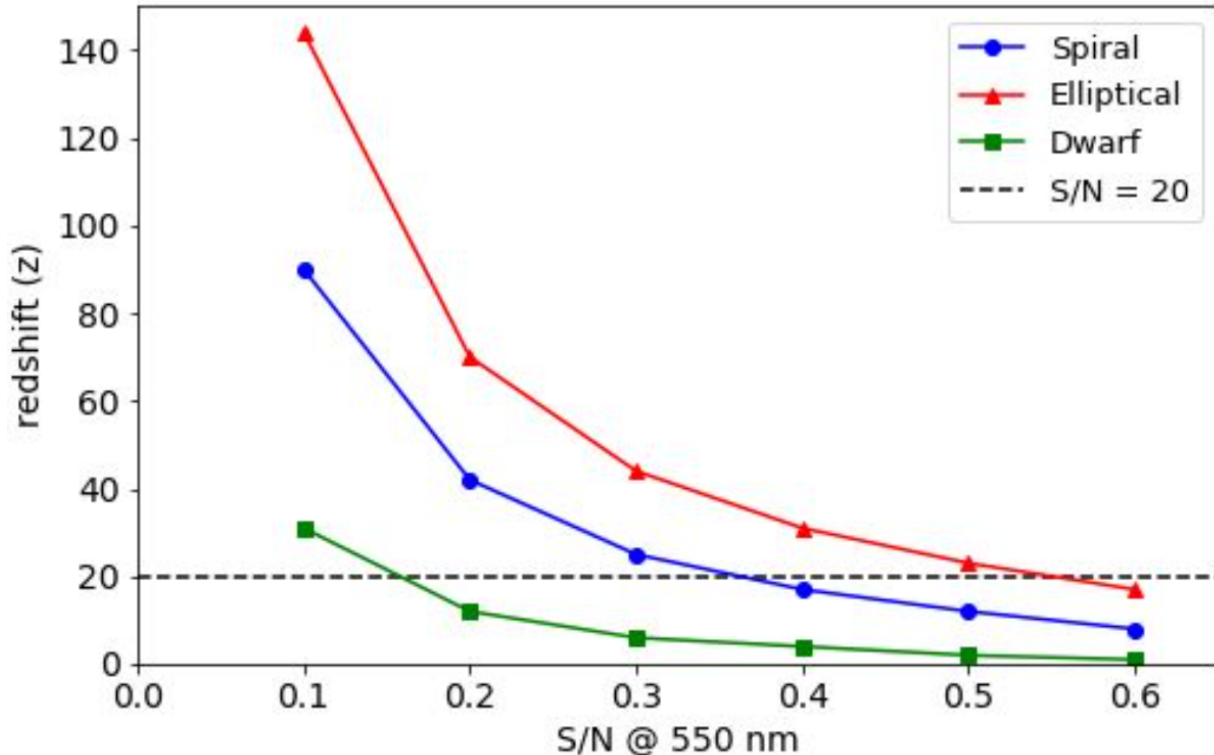
Figure 12. Our simulation of the distribution of the signal-to-noise of spectral region, computed at the wavelength of 550 nm, for different SN-Ia host galaxies as observed by MAAT@GTC. The black dashed line corresponds to our threshold for the signal-to-noise value, useful to obtain reliable results from stellar synthesis population analysis.
