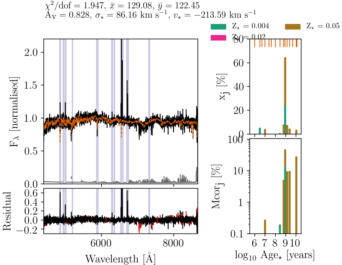
Figure 11. The analysis of the region surrounding GRB 100316D (Izzo et al. in press) using the STARLIGHT (Cid Fernandes et al. 2013) spectral synthesis code. The left panels show the observed spectrum (black line) and the synthetic spectrum obtained from a combination of stellar spectra, whose eigenvalues (depending on the age and metallicities of the eigenvector stellar spectra) are shown in the right panels. The lower left panel shows the residual spectrum, which consists in the nebular component at the GRB location.
